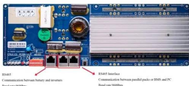
RS485 Communication between battery and inverter Bit rate:9600bps
